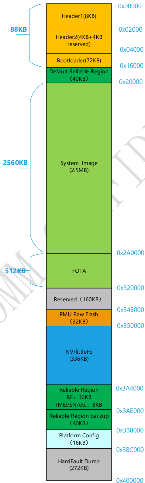
Flash Memory Map
